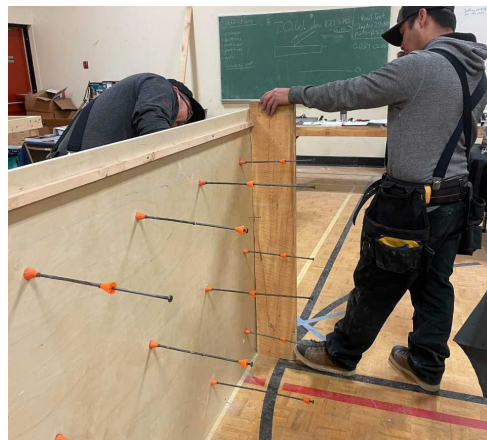
Photo 3: Forming Bulkhead
